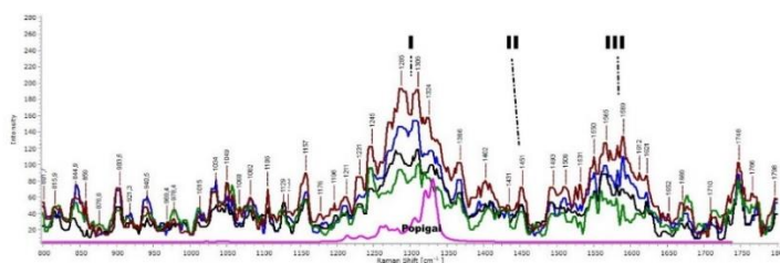
Figure 3. METCCH-diamonds peak wavenumber in D-band (I, around 1308 \text{cm}^{-1} ) II (around 1450 \text{cm}^{-1} ), poor quality D-band; and III (around 1560-1590 \text{cm}^{-1} ) G-band compare
